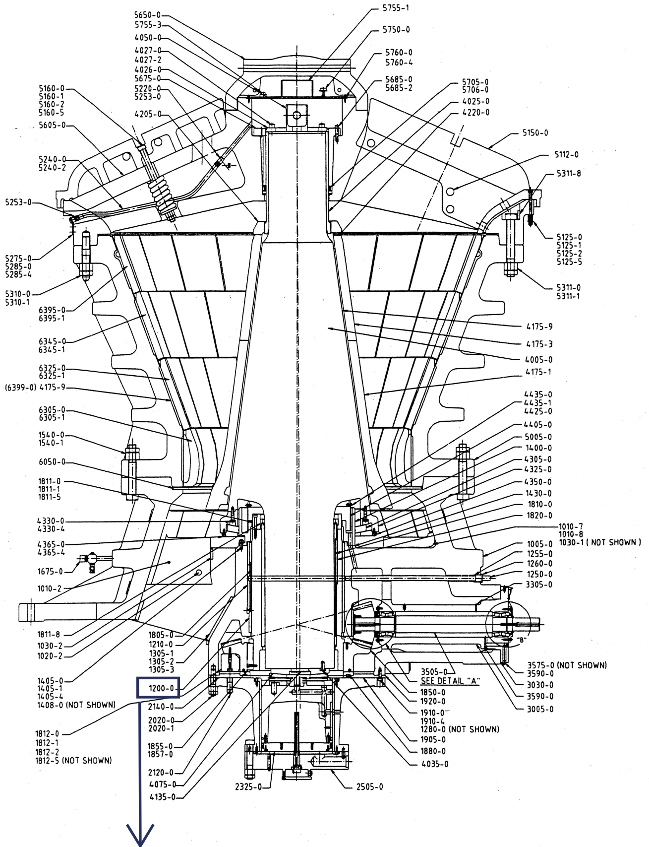
BUSH/SLEEVE BOTTOM SHELL; BRAND: METSO PART NUMBER: 442.4233-01 (CAT NO:1200-0)
